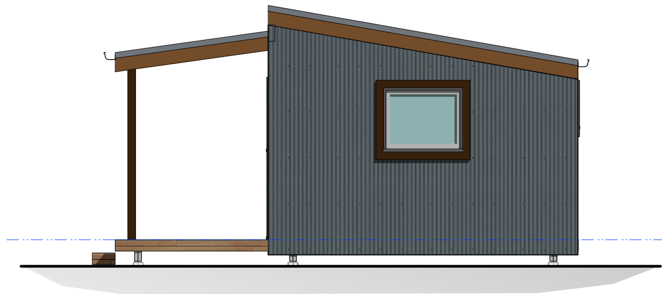
JANE 2 - EAST ELEVATION
