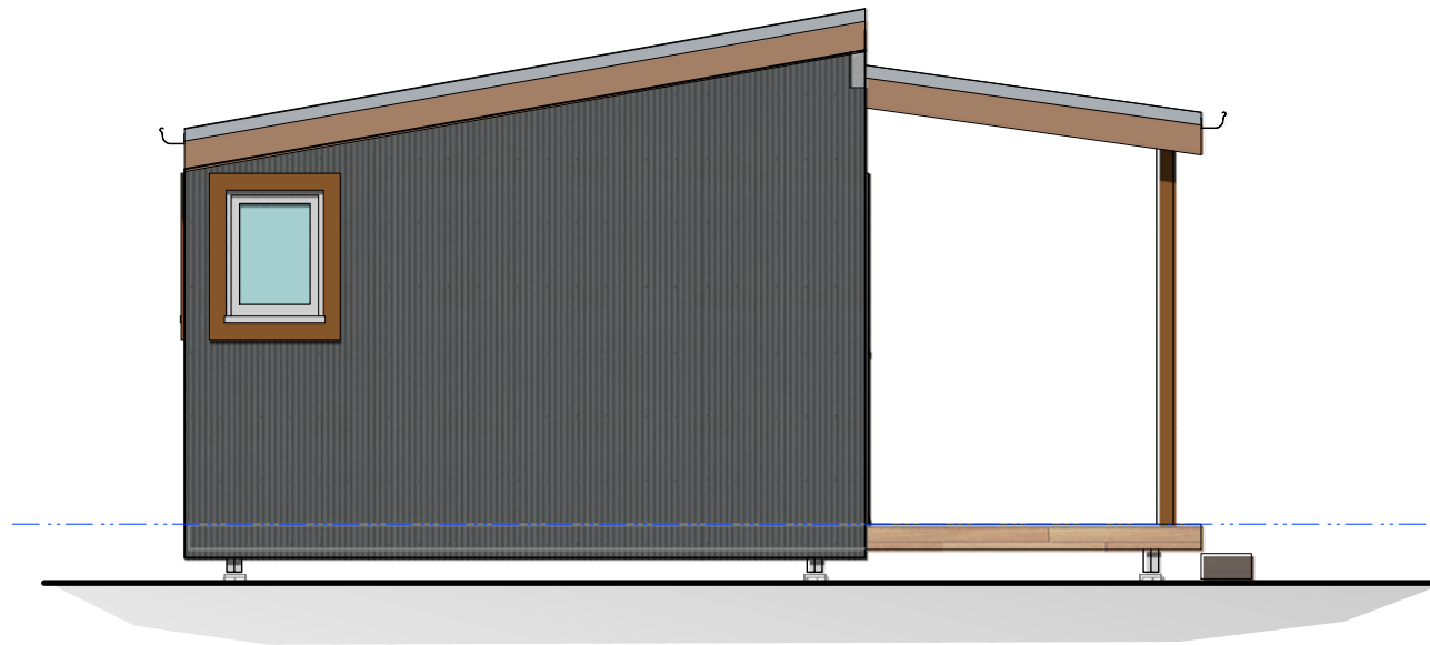
EAST ELEVATION
