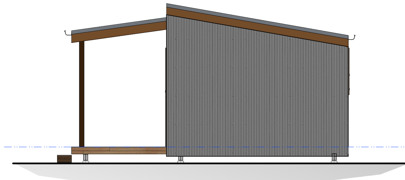
GRANNY - EAST ELEVATION
