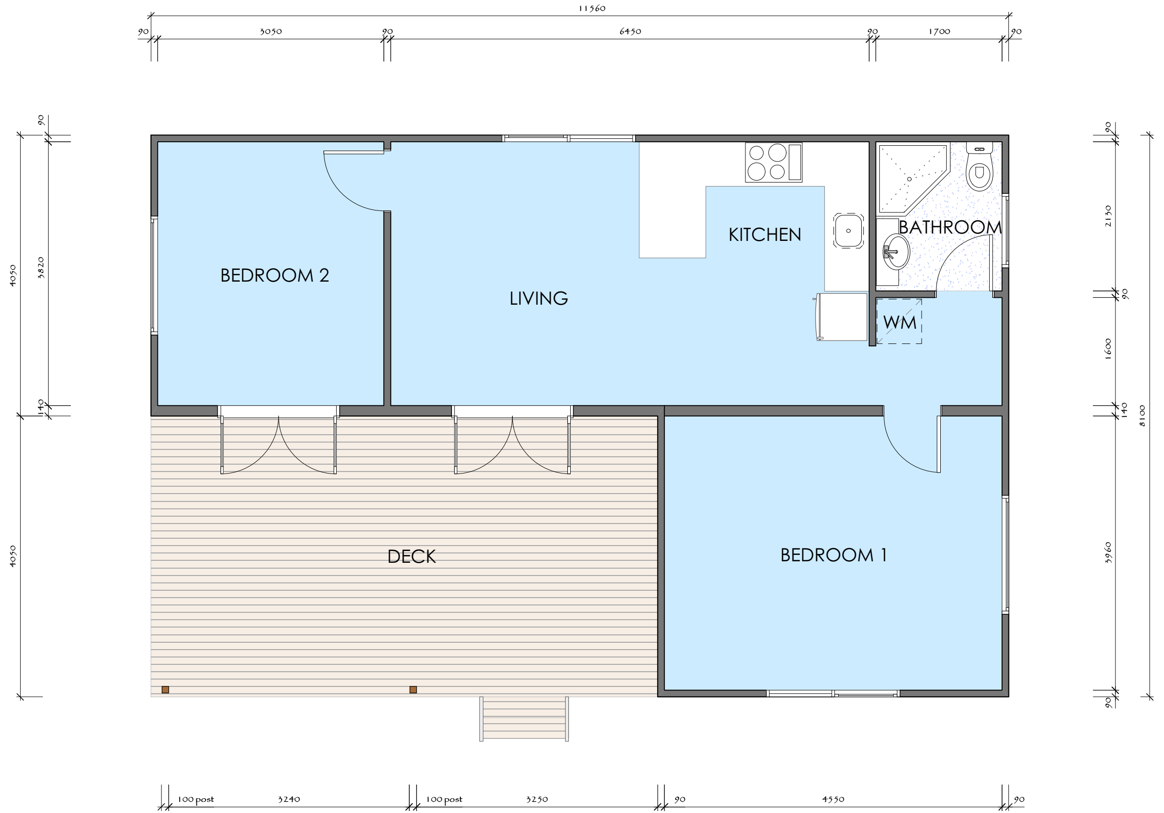
AUSTIN PLUS - FLOOR PLAN
